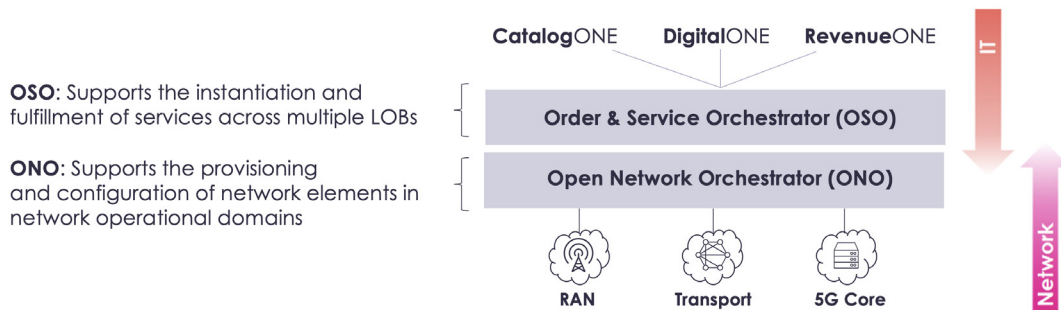
Fig 5 - Amdocs NEO: Open Service & Network Orchestrators
