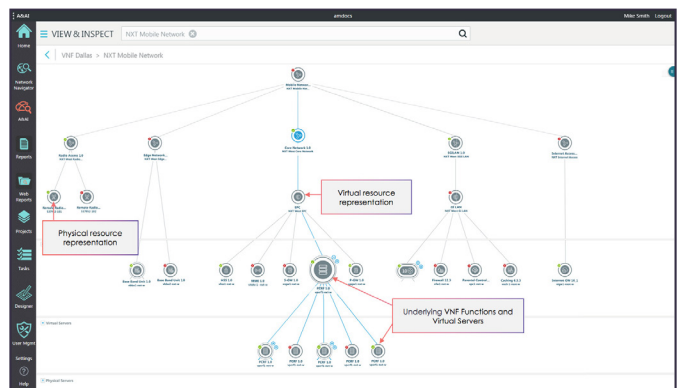
Fig. 7 – Amdocs Open Network Inventory
